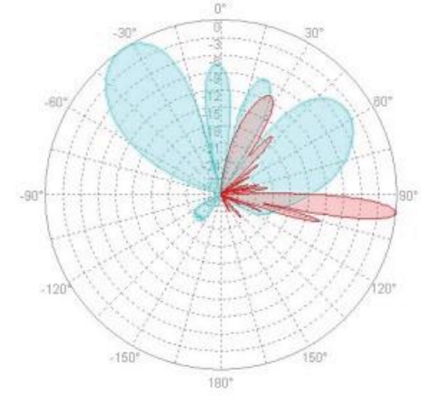
Directional Illustration (30°/3.5GHz)
